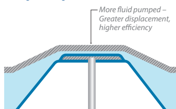
Full-Stroke PTFE Diaphragm During Discharge Stroke
